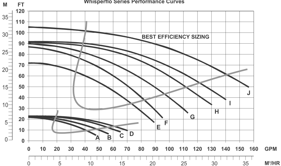
Pentair Pool Products Whisperflo Series Performance Curves
