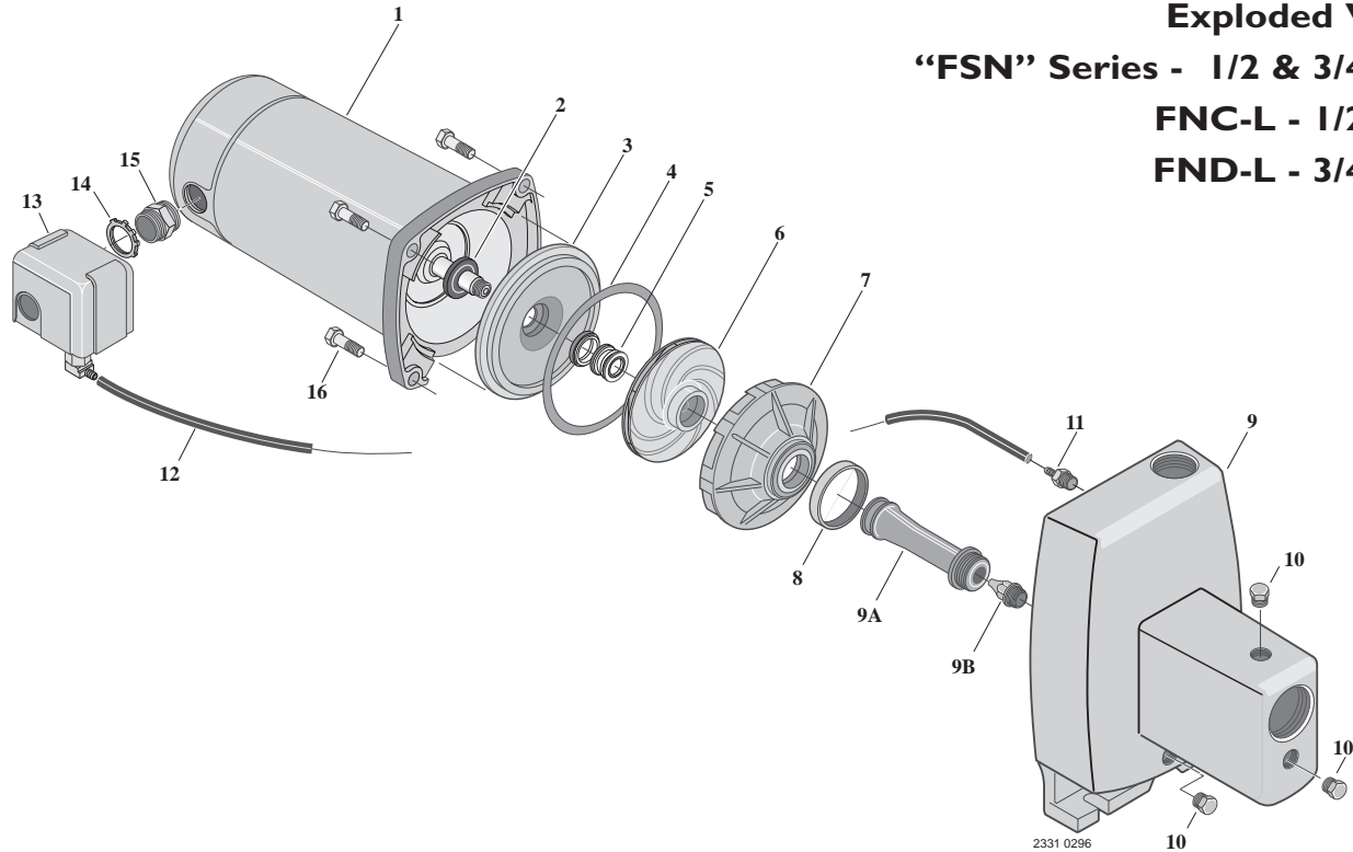
“FSN” Series, 1/2 & 3/4 HP
